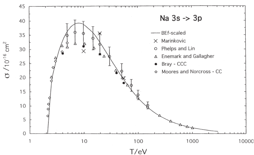
Fig. 1. Sodium 3s\text{-}3p electron-impact excitation cross sections. The solid curve is our scaled plane-wave Born (PWB) result, the solid circles are accurate theoretical results from the convergent close coupling (CCC) method of Bray [12], the diamonds are theoretical results from the close coupling calculation of Moores and Norcross [15], the open circles are experimental results of Phelps and Lin [13] that include corrections for cascading from the upper levels, and the triangles are experimental results of Enemark and Gallagher [14] that are also corrected for cascading. The crosses are experimental results of Marinkovic et al. [29].
