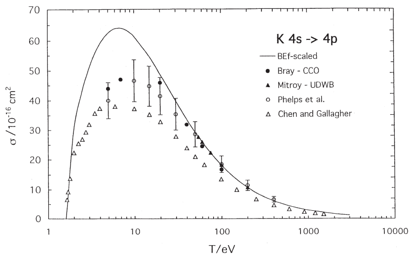
Fig. 2. Potassium 4s\text{-}4p electron-impact excitation cross sections. The solid curve is our scaled plane-wave Born (PWB) result, the solid circles are theoretical results from the coupled-channel optical (CCO) method of Bray et al. [16], the open circles are experimental results of Phelps et al. [17] that include corrections for cascading from the upper levels, and the grey triangles are experimental results of Chen and Gallagher [19] that do not correct for cascading. The solid triangles are theoretical calculations of Mitroy [18] using a unitarized form of the distorted wave Born approximation.
