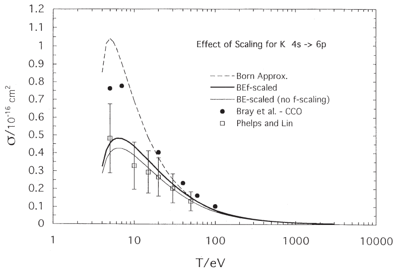
Fig. 6. This figure shows the magnitude of the scaling effect on plane-wave Born cross sections. BE-scaling, Eq. (1), for the 4s-6p transition of potassium decreases the Born cross section by a factor of nearly 3 in the peak region. Adding the f -scaling, Eq. (2), raises the cross section back up by about 10%. Experimental measurements of Phelps and Lin [13] and calculated couple-channel optical results of Bray et al. [16] are also shown.
