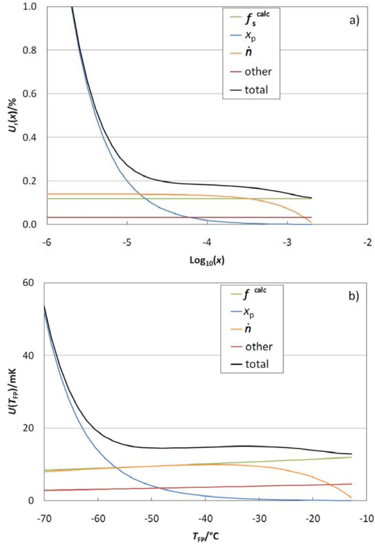
Figure 14. Total expanded uncertainty for the a) water mole fraction (relative uncertainty) and b) frost-point temperature generated by the HHG when it is used in divided flow mode with a saturator pressure of P_s = 300 kPa. ). Here, f_s^{\text{calc}} represents the combined uncertainty contributions from both the saturator and chamber (hygrometer), and \dot{n} represents the combined uncertainty contributions from the wet gas and dry gas.
