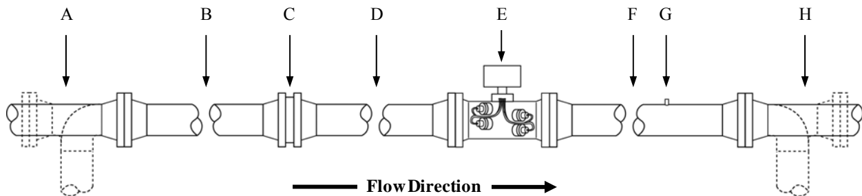
Figure 2. Labeling of uni-directional flowmeter installation configuration (Labels are described in Table 2) This piping configuration meets straight-run requirements for AGA9.
