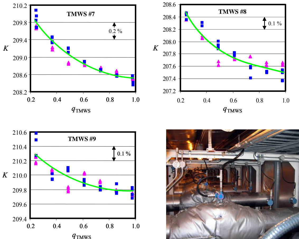
Figure 4.6. K -factor (pulse/m 3 ) calibration curves (—) for all nine TMWS plotted versus volumetric flow (m 3 /s) with the squares (■) denoting the May 2006 data and the triangles (▲) signifying the June 2007 data. (The picture at the lower right shows the nine TMWS.)
