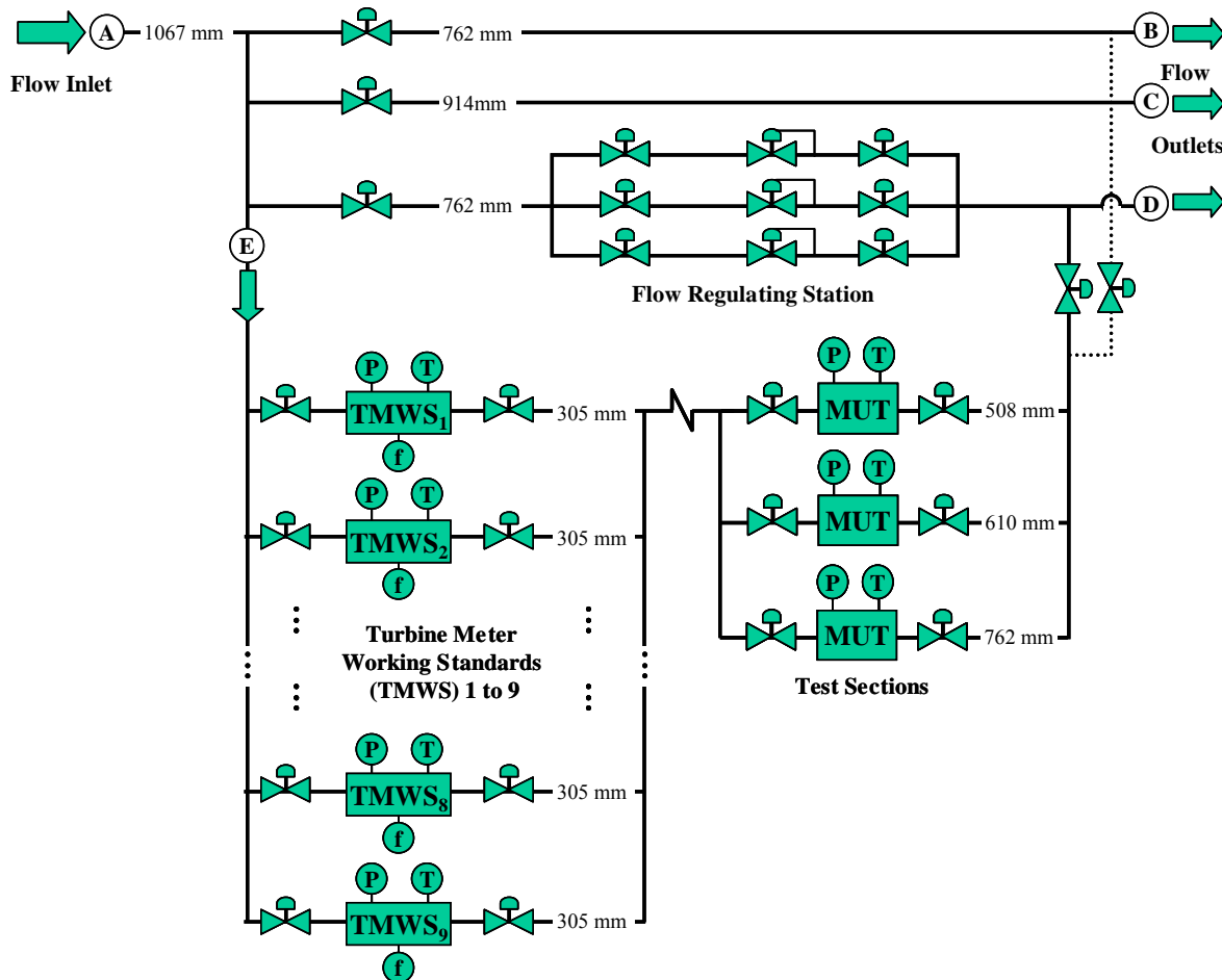
Figure 2.1. CEESI Iowa Flowmetering Facility
