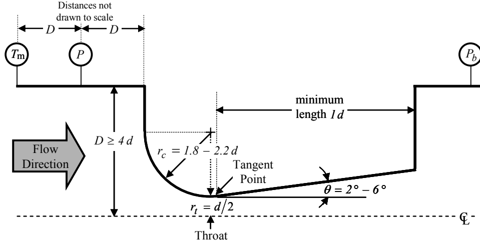
Figure A1. Cross sectional cut of a toroidal shaped ISO 9300 CFV [9]
