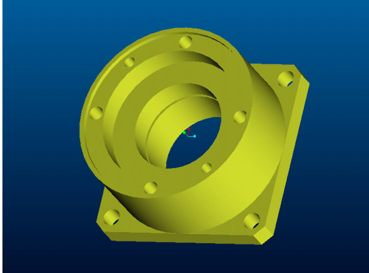
Figure 6 Solid model of the output housing
