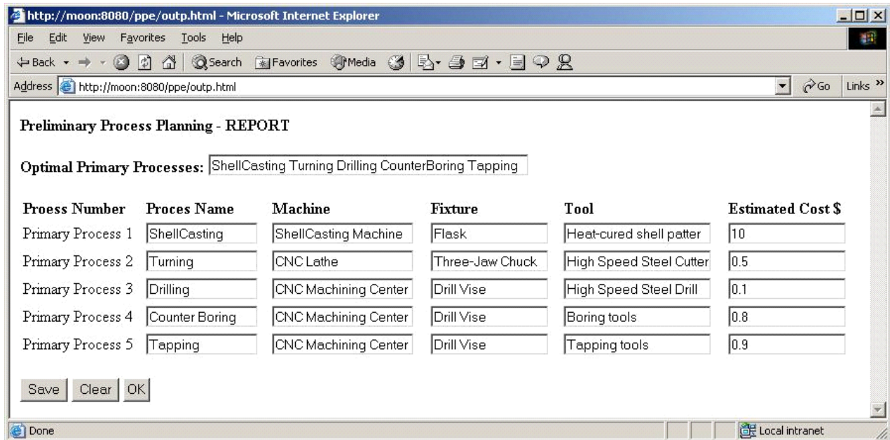
Figure 8 Optimal primary process and resources
