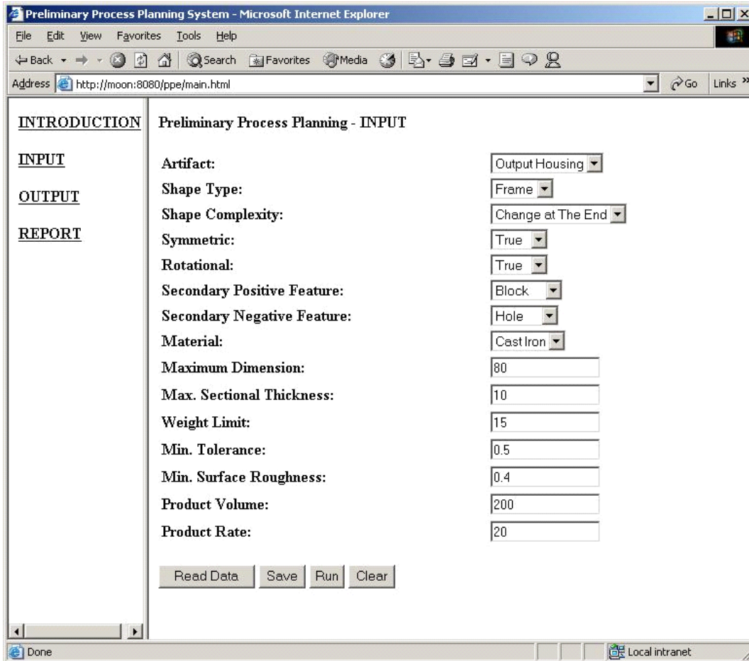
Figure 7 Artifact Information From Database
