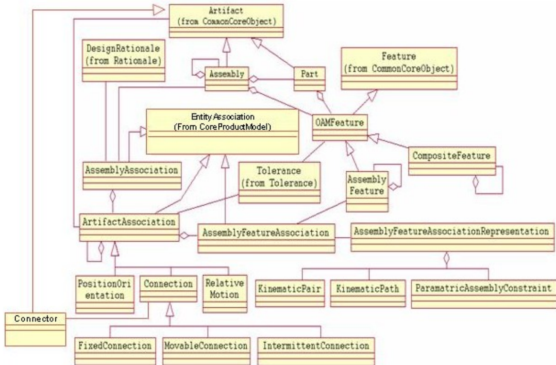
Figure 3: Class diagram of the Open Assembly Model
