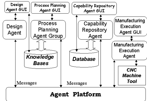
Figure 1 Multiagent system architecture
