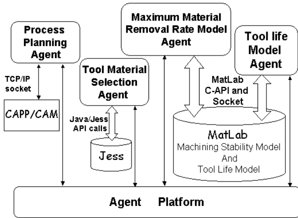
Figure 2 Process planning agent group
