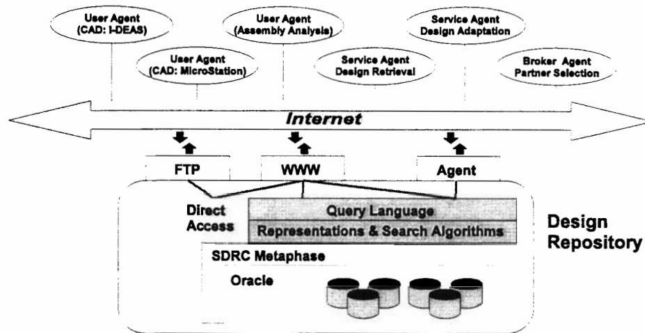
Figure 4: System architecture.
