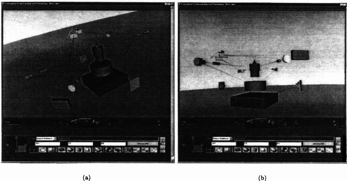
Figure 6: Illustrations of a conceptual design for the missile seeker pictured in Figure 2.
