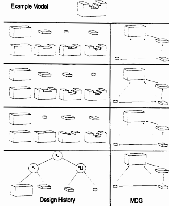
Figure 7: Pictured is a single solid model and several alternative design feature histories and one possible CSG tree that can produce it. On the right are the MDGs for each of these alternatives—note that they are all D-morphic to one another.
