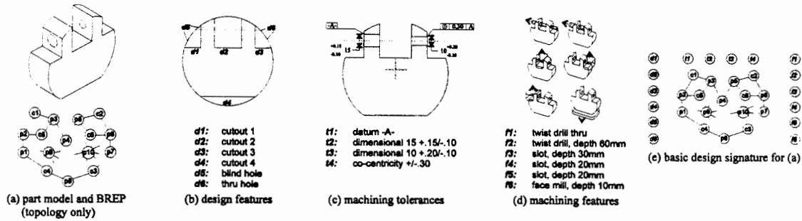
Figure 3: Signature structures: an illustration of (a) a design of a simple bracket and its attributes (b-d) and a design signature (e).
