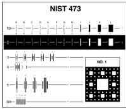
Figure 1. Linewidth Calibration
