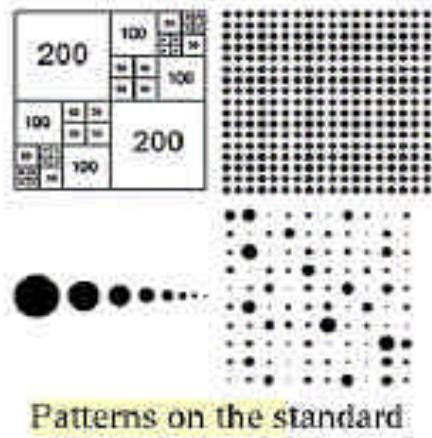
Figure 2. NPL Calibration Target
