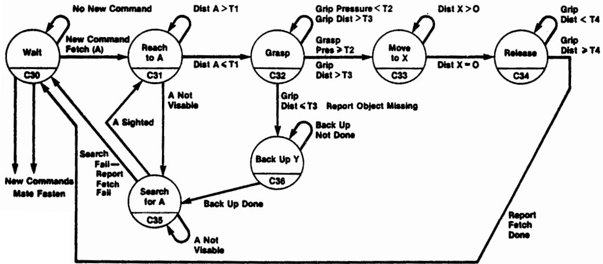
Fig. 3. A state-graph at hierarchical level 3 for a decomposition of the <Fetch (A)> command.
