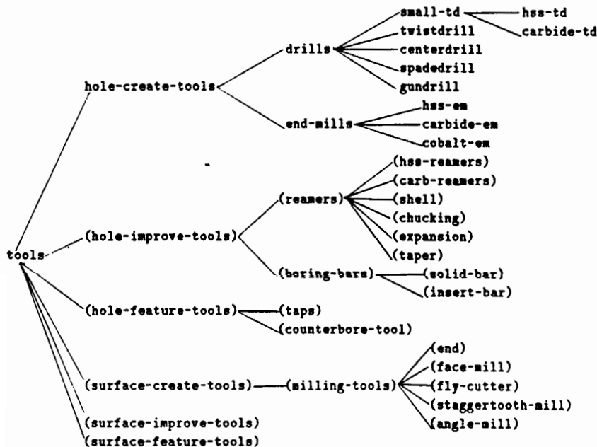
Figure 7: The names of the frames in SIPS's tool hierarchy. The names listed in parentheses have not been put into the hierarchy yet, but will be added soon.
