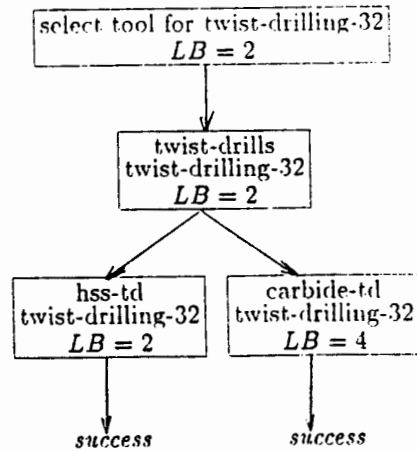
Figure 4: A search space for tool-selection for twist-drilling-32.
