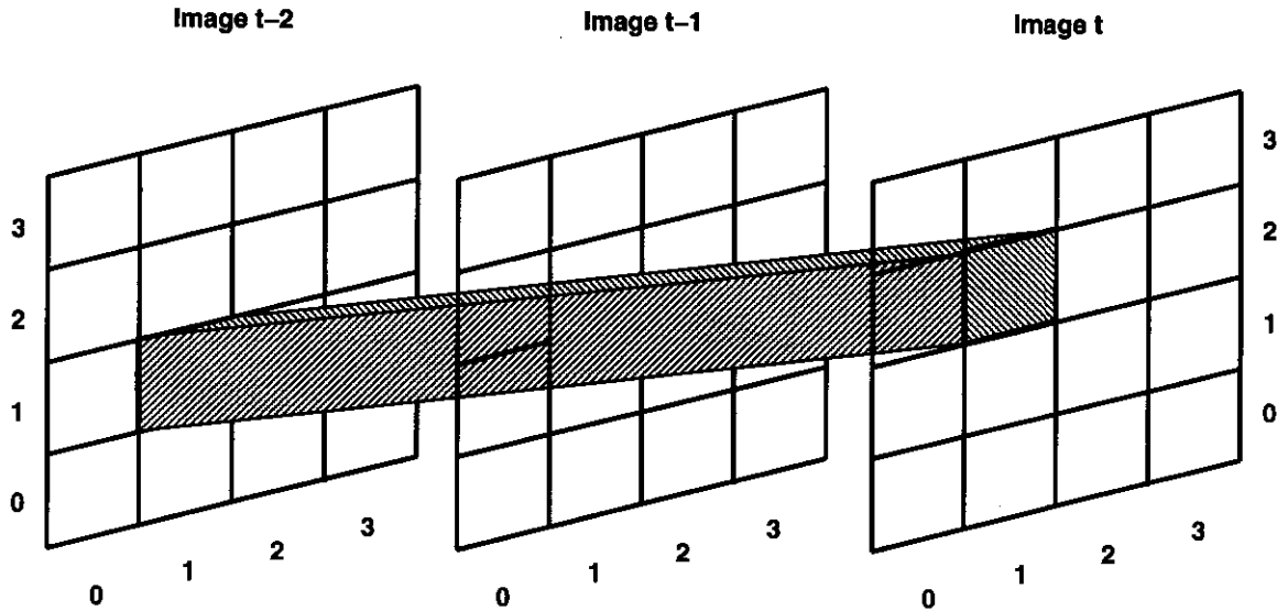
Figure 2: Visualization of motion from Image T - 2 : (1,1) to Image T : (1,2). This would be an optical flow of (0,1/2) pixels per frame motion for pixel Image T : (1,1).
