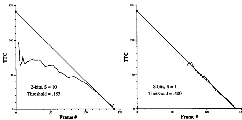
Figure 9: Results of time-to-contact experiment for the collision sequence with (left) 2-bit precision images, S = 10 , lower threshold = 0.183, and (right) full precision images, S = 1 , and lower threshold = 0.400. For the graph on the right, valid measurements did not begin until about halfway through the sequence.
