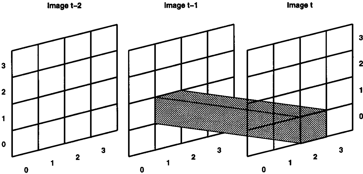
Figure 1: Visualization of motion from Image T - 1 : (1,1) to Image T : (2,0). This would be an optical flow of (1,-1) pixels per frame motion for pixel Image T : (1,1).
