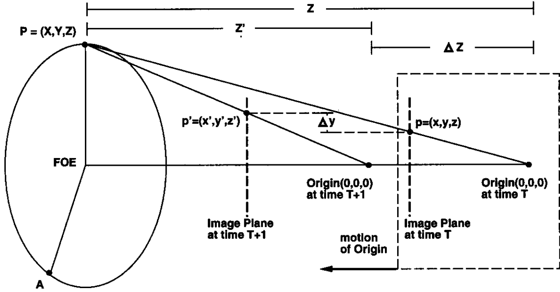
Figure 5: Optical Geometry for time-to-contact. See text for details.
