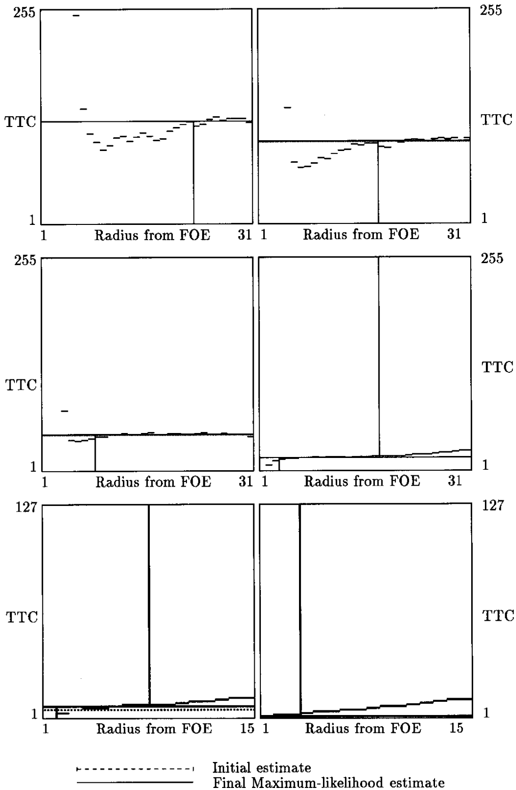
Figure 6: Time-to-contact estimates (in row-major order) for frames 12, 41, 96, 126, 134, and 139. Lower-bound threshold is 0.183 pixels per frame. The plots for the last 2 frames have only a few valid measurements less than 1.0 pixels per frame, so for enhanced visibility the lower left-hand quarter is zoomed in by a factor of 2.
