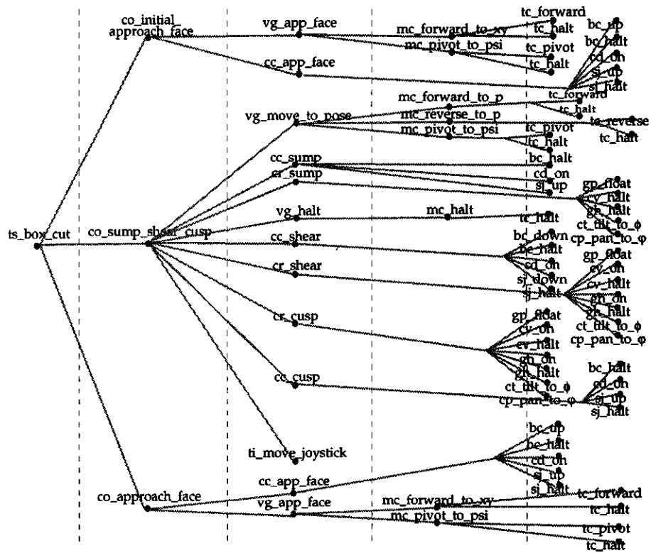
figure 2: Task tree for a box cut of a continuous mining machine
