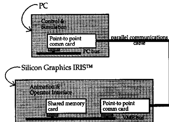
figure 6: Hardware tools
