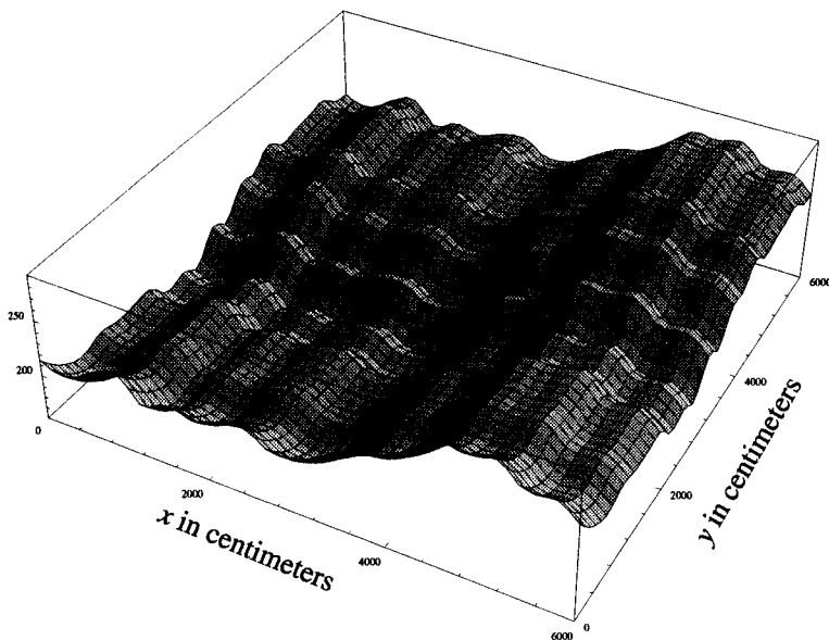
Figure 5: Simulated coal seam height function
