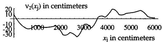
Figure 4: One dimensional random walk functions (interpolated) used in figure 5.
