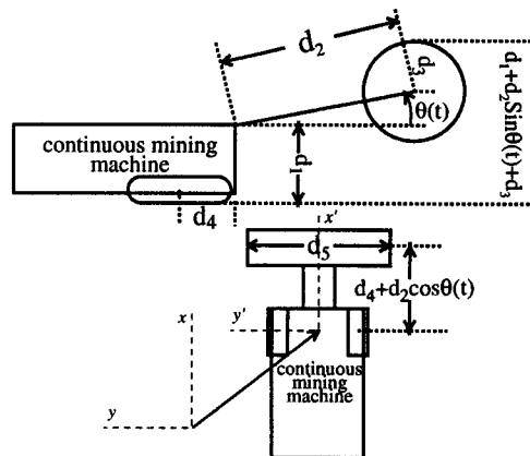
Figure 3: CM dimensions
