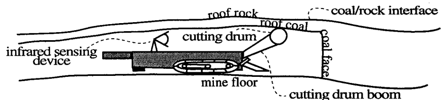
Figure 2: A continuous mining machine in a coal mine.
