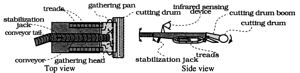
Figure 1: A continuous mining machine and appendages
