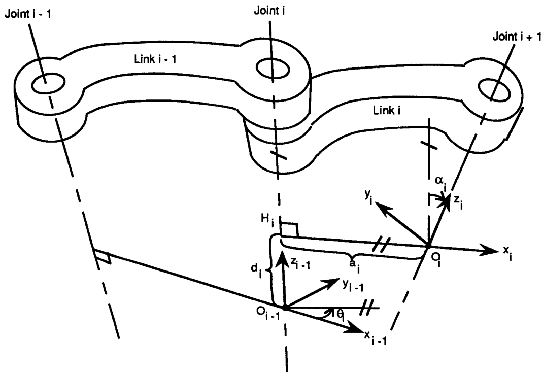
Figure 1: The Denavit-Hartenberg Parameters
