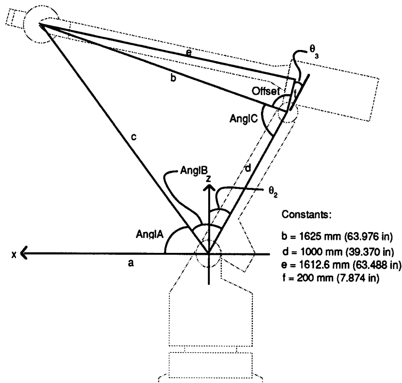
Figure 4: Geometric Solution for Joints 1, 2, and 3
