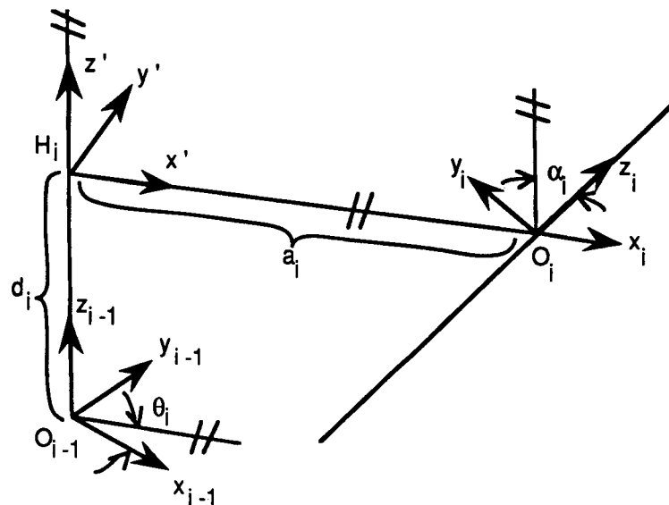
Figure 2: The relationship between adjacent coordinate frames in the Denavit-Hartenberg notation
