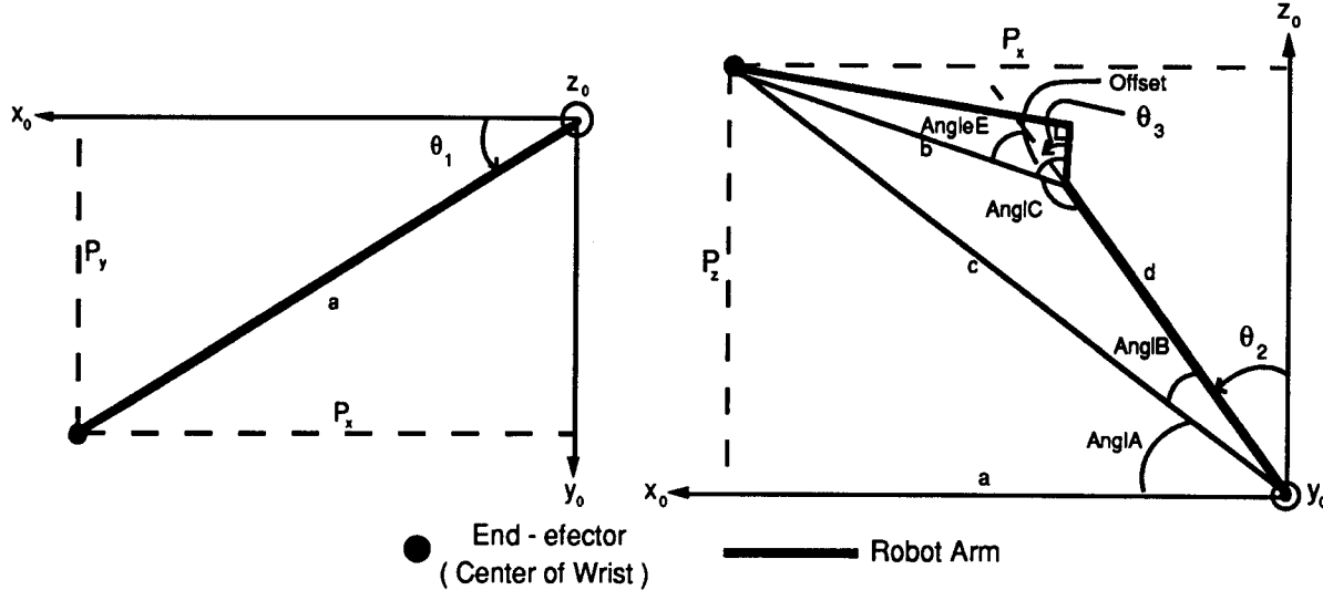
Figure 5: Geometric solution for Joints 1, 2, and 3
