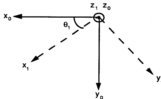
Figure 7: Relative motion of frame 1 with respect to frame 0
