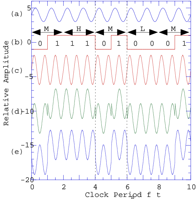
Fig. 4. Input and output waveforms for m = 3, f = f_c . (a) Clock signal [+4 offset]. (b) Digital code signal I_{dc}/I_c and pattern. (c) Sinusoidal drive I_{ac}(t)/I_c [-4 offset]. (d) “In-phase” combined input current [-10 offset]. (e) “Out-of-phase” combined input current with sine wave phase shifted 180^\circ [-16 offset].
