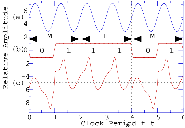
Fig. 2. Simulated input and output waveforms for an example 6 bit code. (a) Sinusoidal drive current I_{ac}(t)/I_c of frequency f=f_s ( m=2 ) [+5 offset]. (b) Digital code bias I_o(t)/I_c . (c) Time-dependent junction voltage V(t)/I_c R showing quantized voltage pulses of different polarity [-5 offset].
