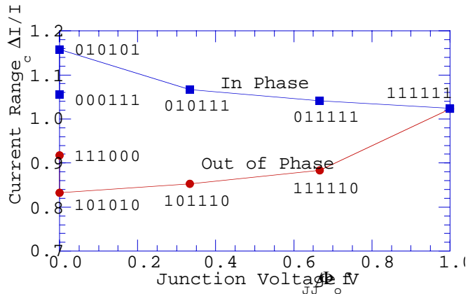
Fig. 6. Current range \Delta I_c vs. junction voltage V_J/(\Phi_s f) for f = f_c , n = 1 . Nine example bit codes are shown for both in-phase and out-of-phase input waveforms.
