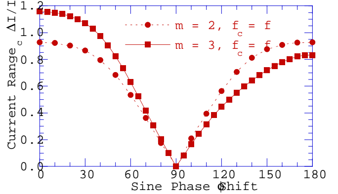
Fig. 5. Current range \Delta I_c vs. sine wave phase shift \phi relative to the digital code signal for m = 2 and m = 3, f = f_c, n = 1, I_{ac} = 2.17I_c, \pm I_o = \pm 1.07I_c , and the periodic 01 pattern.
