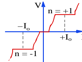
Fig. 1. Simulated voltage-current curve of a sinusoidally driven resistively shunted Josephson junction with constant voltage steps.
