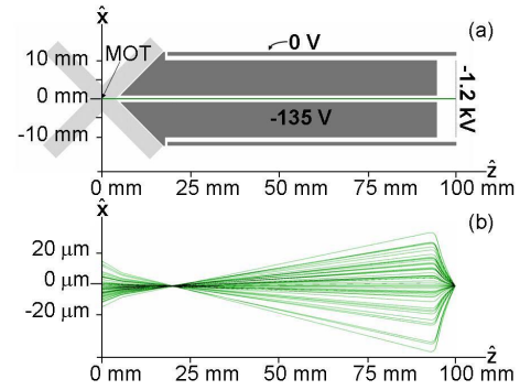
FIG. 1. (Color online) Lens geometry used in ray tracing simulations. (a) Scale drawing, showing electrostatic lens elements (dark gray) and MOT laser beams (light gray). The lens consists of three elements: a tapered cylinder held at -135 V, a grounded sheath surrounding the tapered cylinder, and a back plane held at -1.2 kV. At this scale, the atomic cloud is a small spot at the origin, and the ion trajectories lie along the horizontal axis ( x=0 line). (b) Typical ion trajectories, with vertical axis expanded by a factor of 365. These trajectories, in green, were calculated for a MOT with a standard deviation of \sigma_x=\sigma_y=\sigma_z=5 \mu m and temperature of 100 \mu K. For clarity, only 50 of the 10 000 trajectories calculated are shown.
