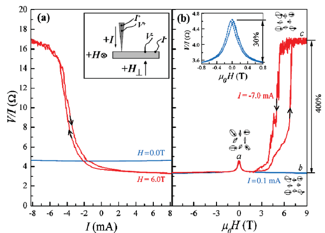
FIG. 1 (color). (a) Resistance vs current in 0 T (blue) and 6 T (red) of a contact on granular \text{Co}_{18}\text{Ag}_{82} (sample #12) at 4.2 K; inset shows schematics of point-contact measurement. (b) Magnetoresistance (MR) of 30% (blue) using currents 0.1 mA and 400% (red) MR at -7 mA of the same contact as in (a), and the schematic spin structures at a , b , and c ; the inset shows MR in small fields.
