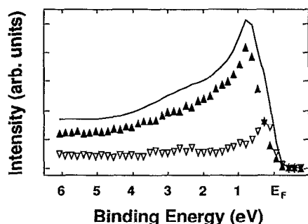
FIG. 7. Normal emission photoemission spectra from Fe(001) at \theta_i = 70^\circ and h\nu = 60 eV.
