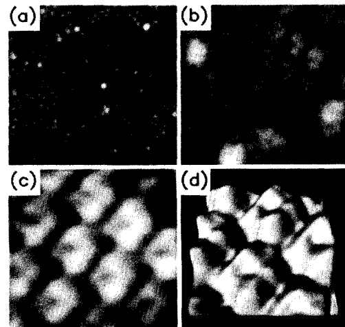
FIG. 1. STM gray-scale topographic images (filled states), with increasing magnification, of a 2D Cs overlayer on room temperature InSb(110): (a) 400 \times 400 Å 2 ; (b) 100 \times 100 Å 2 ; (c) 50 \times 50 Å 2 ; (d) 30 \times 30 Å 2 (rendered as a solid, in perspective). (b)-(d) zoom in on a c(2\times 6) ordered area composed of planar Cs clusters. Each cluster appears to have four Cs atoms, topographically \approx 1 Å high. The Cs coverage, as estimated from the images, is \approx 0.5 Cs per InSb(110) unit cell ( 1.7 \times 10^{14} cm -2 ). Note that the +x scan direction is approximately 45° from the [1\bar{1}0] direction, and that the dimensions are uncorrected for thermal drift.
