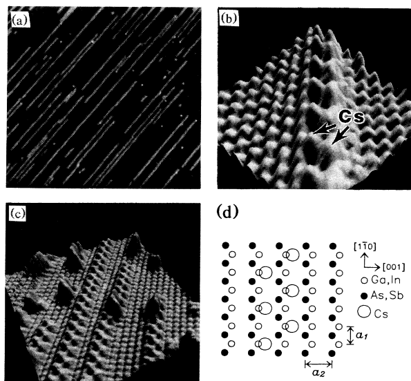
FIG. 1. STM images recorded with negative sample bias: (a) 1370 \times 1370 \text{ \AA} ( \sim 0.03 \text{ ML} ), 1D Cs zig-zag chains on GaAs(110); (b) 70 \times 70 \text{ \AA} , a single Cs zig-zag chain on GaAs(110); (c) 200 \times 200 \text{ \AA} , Cs zig-zag chains on InSb(110). (d) Schematic drawing of the Cs zig-zag chains; the lattice constants for GaAs (InSb) are a_1 = 4.00 ( 4.58 ) \text{\AA} and a_2 = 5.65 ( 6.48 ) \text{\AA} . The grey scale in the images corresponds to a range of approximately 1.5 \text{ \AA} .
