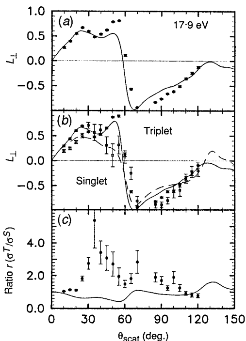
Fig. 3. Spin-polarised superelastic scattering from Na(3P) at 17.9 eV incident energy versus scattering angle \theta_{\text{scat}} : (a) Unpolarised measurement of angular momentum transferred perpendicular to the scattering plane, L_{\perp} . (b) Singlet (squares) and triplet (circles) perpendicular angular momentum transfer, L_{\perp}^S and L_{\perp}^T . (c) Ratio r of triplet to singlet cross sections.
