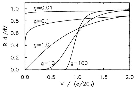
FIG. 2. The current-voltage characteristics of a tunnel junction connected to an infinite, lossless transmission line of impedance Z = gR_H/2 . R is the asymptotic value of (dI/dV)^{-1} . The curves were calculated at zero temperature in the limit that the junction impedance R goes to infinity.
