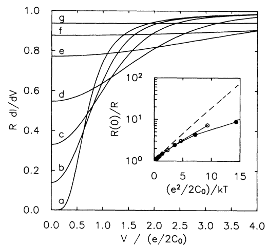
FIG. 3. The current-voltage characteristics of a tunnel junction connected to a resistive transmission line at finite temperature. The curves a - g are for temperatures 0, 0.5, 1.0, 2.0, 5.0, 10, and 20 K. The parameters are junction capacitance C_0 = 0.2 fF, specific resistance r = 8000 \Omega/\mu\text{m} , specific capacitance c = 0.02 fF/ \mu\text{m} , and specific inductance l = 600 fH/ \mu\text{m} . Inset: The values of R(0)/R plotted vs the charging energy over the temperature for these same curves (open circles). The dashed line gives the semiclassical result. The solid circles show R(0)/R for a series of junctions at constant temperature T = 1.3 K as the junction capacitance is varied over C_0 = 0.05, 0.1, 0.2, 0.5, 1, 2, 5, 10 , and 20 fF.
