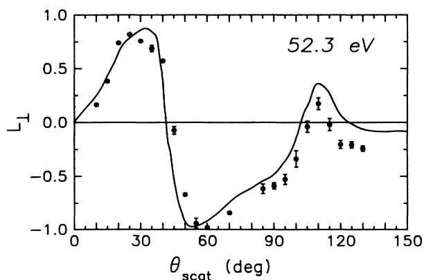
FIG. 6. Superelastic scattering from Na(3P) at 52.3 eV incident energy vs scattering angle \theta_{\text{scat}} . Unpolarized measurement of angular momentum transferred perpendicular to the scattering plane L_{\perp} . Solid circles, present work; solid line, four-state close-coupling calculation of Mitroy et al. (Ref. 20).
