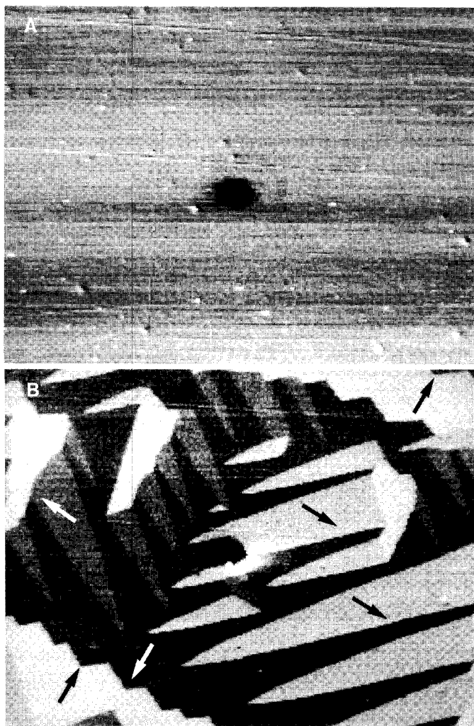
Fig. 5. (A) A conventional SEM micrograph of the surface of an Fe-3%Si crystal ( x -axis length, 100 \mu\text{m} ). (B) The simultaneously obtained map of the domain structure of the same region. There are four in-plane, easy axes of magnetization due to the cubic lattice anisotropy. The four gray levels indicate the four possible domain orientations, as indicated by the arrows. The domains are unaffected by most of the surface defects or scratches but are modified by the large defect at the center of the image.
