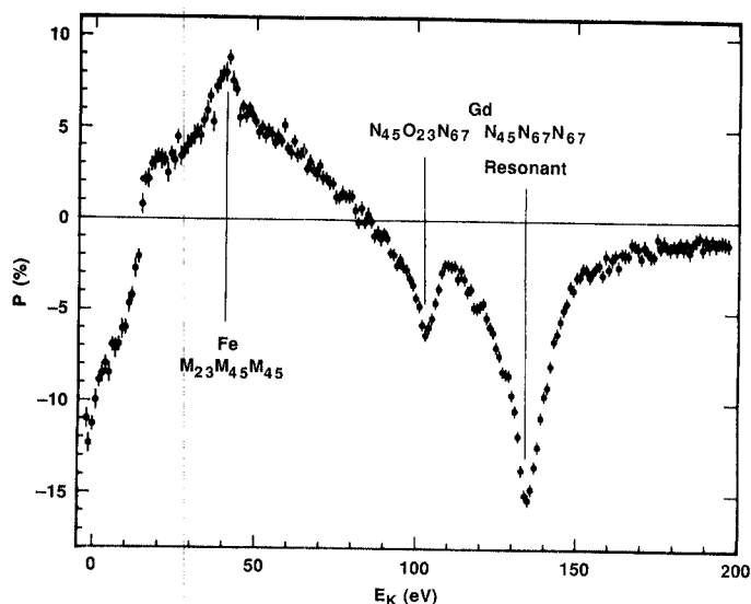
Fig. 3. The secondary electron spin polarization as a function of kinetic energy for a one-monolayer gadolinium film on an Fe(100) crystal surface. The primary energy was 2500 eV, and the measurement temperature was 150 K. Auger transitions originating in iron and gadolinium yield polarizations of opposite sign, indicating an antiferromagnetic coupling of the gadolinium layer to the iron. [From (22)]
