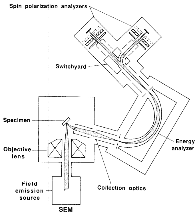
Fig. 4. A schematic view of the scanning electron microscope with two orthogonal spin analyzers to measure all three components of the electron spin polarization. The detectors and the optional energy analyzer are shown much larger than scale for clarity. [From (27)]
