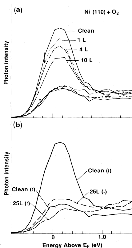
FIG. 2. Spin-resolved photon-intensity spectra, N_{\uparrow} and N_{\downarrow} , measured at room temperature and 25^\circ angle of incidence of the spin-polarized electron beam. The spectrum of the clean Ni(110) surface is compared to surfaces with oxygen exposures of (a) 1, 4, and 10 L, and (b) 25 L.
