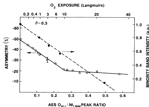
FIG. 3. Asymmetry parameter A = (N_{\uparrow} - N_{\downarrow}) / (N_{\uparrow} + N_{\downarrow}) (left-hand scale) and minority-band intensity N_{\downarrow} (right-hand scale) as a function of the Auger [O(511 eV)/Ni (848 eV)] (dN/dE) peak-to-peak ratio. The coverage scale in monolayers was set taking \Theta = 0.3 at 1 L exposure, where the (2 \times 1) pattern is observed (Ref. 8).
