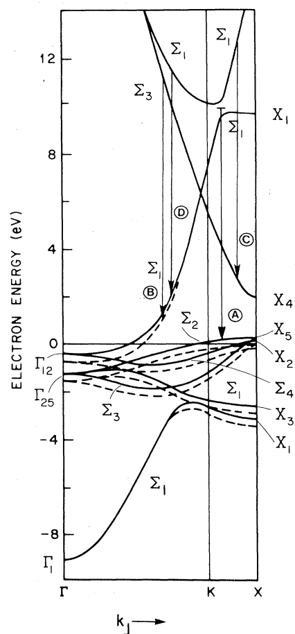
FIG. 1. Band structure of Ni along the direction normal to the Ni(110) surface. The arrows show possible 9.7-eV transition. Dashed curves distinguish the majority-spin bands.
