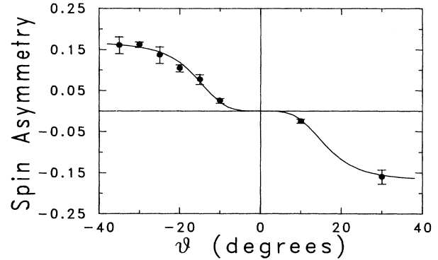
FIG. 2. Spin asymmetry (N_{\uparrow} - N_{\downarrow}) / (N_{\uparrow} + N_{\downarrow}) in superelastic scattering as a function of scattering angle \theta . The laser is linearly polarized parallel to the incident electron direction ( \beta = 0 ). Positive scattering angle corresponds to scattering to the left. An antisymmetric curve is drawn to guide the eye.
