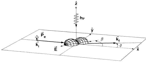
FIG. 1. Schematic of the scattering geometry, showing a representation of the charge density of the prepared 3P state. Electrons with spin polarization \mathbf{P}_e perpendicular to the scattering plane are incident with momentum \mathbf{k}_i , and scatter into an angle \theta with momentum \mathbf{k}_f . The initial atomic state is prepared with linearly polarized laser light incident perpendicular to the scattering plane. The electric vector \mathbf{E} of the light makes an angle \beta with the incident electron direction.
