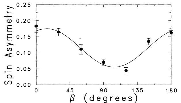
FIG. 3. Spin asymmetry (N_{\uparrow} - N_{\downarrow}) / (N_{\uparrow} + N_{\downarrow}) in superelastic scattering vs laser polarization angle \beta . The scattering angle is -30^\circ . \beta = 0 corresponds to the incident electron direction. The curve is a least-squares fit of the function A + B \cos(2\beta + C) . The parameters A , B , and C have the values 0.115 \pm 0.006 , 0.060 \pm 0.008 , and -28^\circ \pm 9^\circ .
