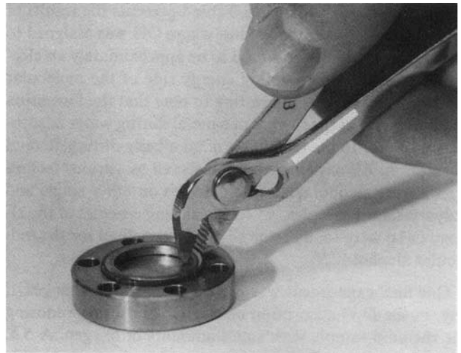
FIG 2. Tool positioned for removal of Miniconflat gasket.
