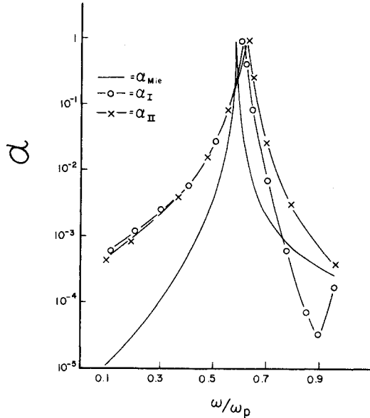
FIG. 1. Plot of the absorption of a sphere with radius R = 25 \text{ \AA} , electron density r_s = 4 , and scattering time \omega_p \tau = 10^3 . \alpha_{\text{Mie}} is the adsorption given by Mie theory and includes only transverse mode excitation. \alpha_I and \alpha_{II} include e-h excitations as well as plasmons and transverse modes and are calculated from two different forms of the ansatz. They are given by Eqs. (5.10) and (5.22), respectively.
