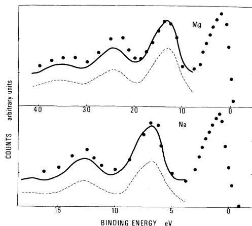
FIG. 1. Comparison of theory and experiment for the XPS valence-band loss spectra of Mg and Na. The dots represent experiment. The solid line is the complete theory and the dashed line is the theory without intrinsic plasmons and intrinsic electron-hole pairs. The no-loss peaks are taken from experiment and serve as input data for the calculations of the loss spectra.
