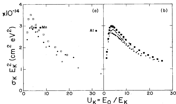
FIG. 4. Experimental values of \sigma_K E_K^2 as a function of U_K . (a) Solid circles denote data of Pockman et al. (1947) for Ni; solid squares denote data of Fischer and Hoffman (1967) for Al, Mn, and Cu; the open squares denote the results of Hink and Ziegler (1969) for Al; and the open circles denote the results of Hink and Paschke (1971a, 1971b) for C. (b) Results of Glupe and Mehlhorn (1967, 1971), of Glupe (1972), and of Bekk (1974) for C (triangles), Ne (crosses), N (squares), and O (circles).
