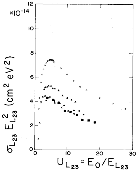
FIG. 6. Experimental values of \sigma_{L_{23}} E_{L_{23}}^2 as a function of U_{L_{23}} . The solid symbols are the data of Vrakking and Meyer (1974) for P (squares), S (circles), and Cl (triangles); the crosses are the data of Ogurtsov (1973) for Ar; and the open circles are the data of Christofzik (1970) for Ar.
