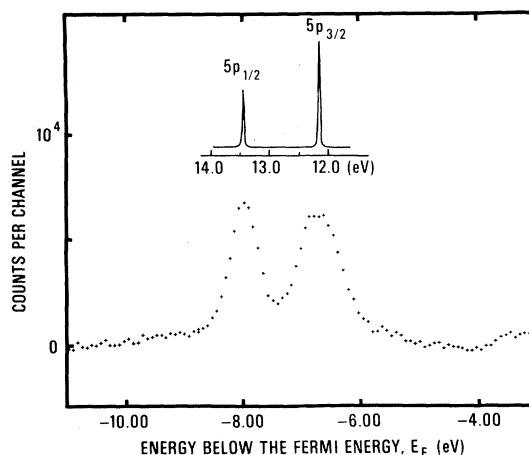
FIG. 2. Expanded view of the two Xe 5p peaks from the difference spectrum of Fig. 1. The inset is the photoelectron distribution for gaseous Xe (Ref. 5).
