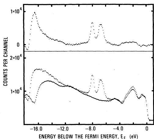
FIG. 1. Photoelectron energy distributions. The lowermost curve is for W(100) at a temperature of \sim 80 K, and directly above it is the distribution after exposure to 5 Langmuirs of xenon. The difference of the two distributions is given at the top of the figure.
