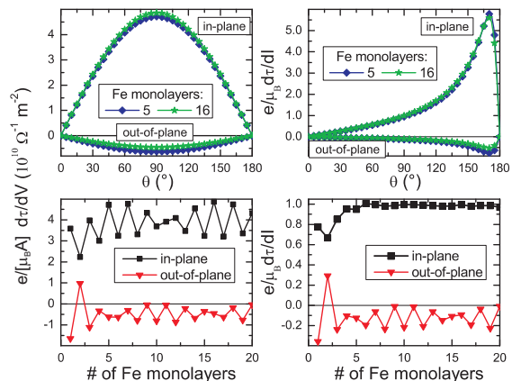
FIG. 2: (Color online) Top: Torkance (left) per in-plane unit cell area A and torque per current (right) acting on the free layer as a function of the relative angle \theta between the magnetizations of the Fe layers. Results are shown for different thicknesses of the free layer as indicated in the figure. Bottom: Torkance (left) and torque per current (right) as a function of the free layer thickness for an angle of 90^\circ . All calculations have a 20 monolayer fixed layer and a 6 monolayer barrier.
