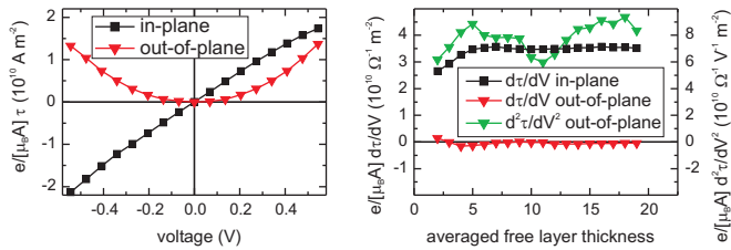
FIG. 4: (Color online) Non-linear bias dependence of the torque per in-plane unit cell area A for samples with thickness fluctuations. We assume an average free layer thickness n consisting of 50 % n , 25 % (n + 1) , and 25 % (n - 1) Fe monolayers. The fixed layer consists of equal parts 19 monolayers and 20 monolayers of Fe. The total torque is calculated by conducting the possible six junctions in parallel. Left: Bias dependence of the torque for a averaged free layer thickness of 19 monolayers. Right: Torkance and derivative of the torkance as a function of the averaged free layer thickness. Note that the scale is identical to the scale in the bottom left panel of Fig. 2.
