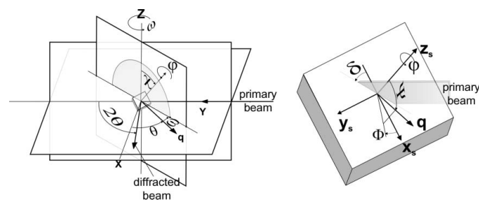
Figure 1 Diffraction geometry in a four-circle configuration. The primary beam should be pictured as rectangular, and it is within the YZ plane (typical beam dimensions Z = 3 mm, X = 0.04 mm). On the right, the magnified specimen is shown. The z_s axis is parallel to the \varphi axis. The azimuth \Phi is the angle between x_s and the normal projection of the scattering vector q onto the specimen surface. The tilt \Psi is the angle between z_s and q . The angle \delta introduced here is the rotation of the beam spot at \varphi = \text{constant} with respect to (\omega + \theta) = 90^\circ where \delta = 0 .
