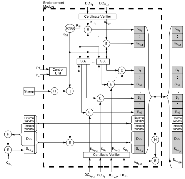
Figure 9: Complete Encryption Module
