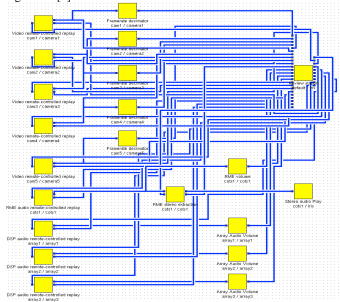
Figure 2- Executable Smart Data Flow System graph for Meeting Room data processing and review.
