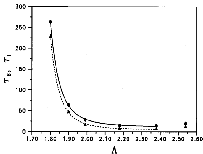
FIG. 10. Induction time \tau_I and thread breakup time \tau_B vs \Lambda . Lines are fit to Eq. (9) and (10). The solid line and the dotted line are fits to the breakup and the induction times given by Eqs. (9) and (10), respectively. The relatively small difference between these times reflects the long induction times where the thread is “thinking” about breaking up.
