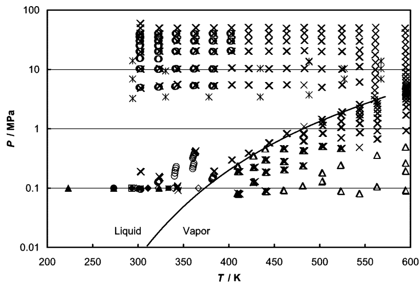
Figure 1. Distribution of the data for the thermal conductivity of methylcyclohexane: ×, transient (Pt); O, transient (Ta); Δ, steady state (Pt); *, Perkins; 14 ◇, Mallan et al.; 15 ▲, Jamieson and Cartwright; 16 ●, Parkinson; 17 ◆, Sakiadis and Coates; 18 □, Briggs; 19 ■, Smith. 20 The solid line shows the vapor–liquid saturation boundary and terminates at the critical point 1 (572.2 K and 3.47 MPa).
