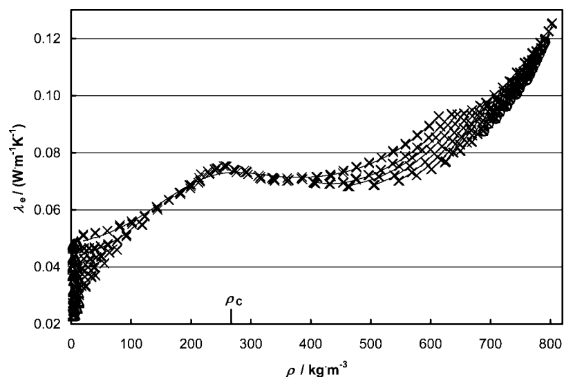
Figure 2. Thermal conductivity of methylcyclohexane as a function of the density calculated at the measured temperature and pressure: ×, transient (Pt); O, transient (Ta); Δ, steady state (Pt); solid lines given by the correlation developed in this work.
