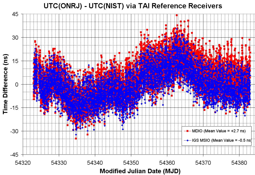
Figure 8. UTC(NIST) – UTC(ONRJ) with MDIO and MSIO corrections applied.
