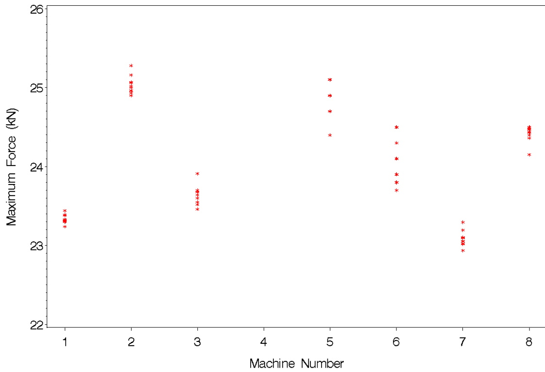
Figure 13. Maximum force for seven Charpy machines at the high energy level.
