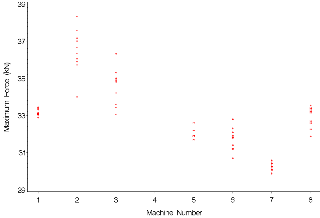
Figure 12. Maximum force for seven Charpy machines at the low energy level.
