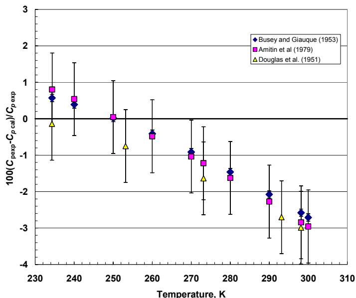
Figure 10a. Comparison of heat capacities calculated with eq (1) and eq (2), subject to the constraint that the vapor pressure data of Knudsen be represented to within 2 %, with experimental heat capacity data.
