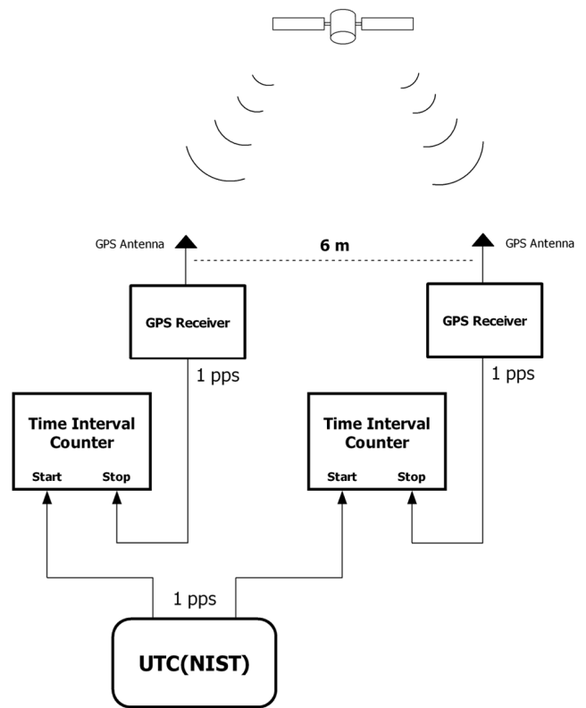
Figure 3. A common-view, common-clock delay calibration.
