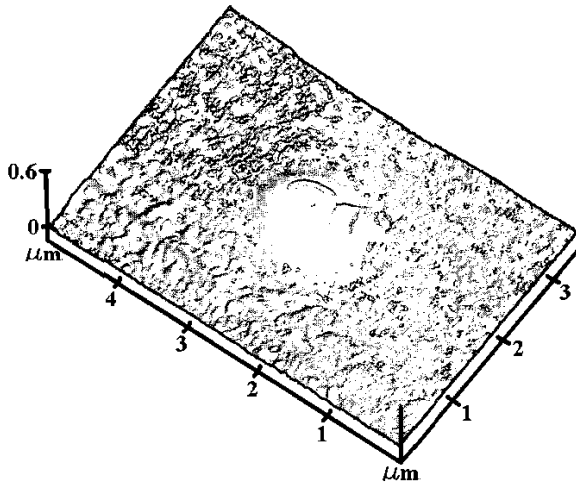
Figure 1: 3D AFM scan of EBD on a silicon surface. Height is approximately 0.6 \mu\text{m} .
