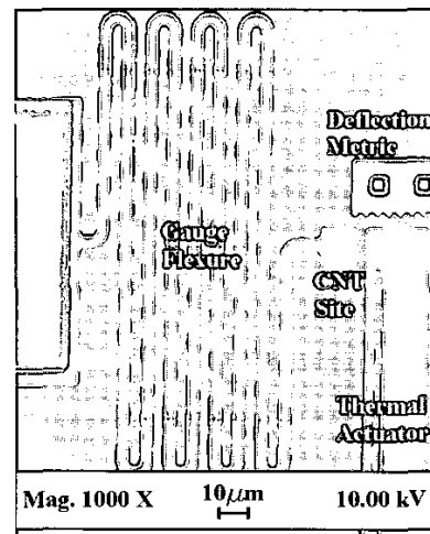
Figure 4: Tensile testing device for CNTs.
