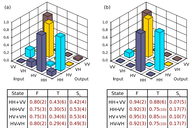
FIG. 3 (color online). (a) Experimentally measured truth table for the CNOT gate in the logical basis (data represent coincidence counts minus accidental counts due to Raman noise and detector dark counts). The highest peak values are: 0.81 \pm 0.05 (VV, VV), 0.85 \pm 0.06 (VH, VH), 0.94 \pm 0.07 (HV, HH), and 0.88 \pm 0.06 (HH, HV). Also shown is the Bell-state characterization for the same gate. Fidelity ( F ), tangle [ T \equiv (\text{concurrence})^2 ], and linear entropy ( S_L \equiv \frac{4}{3}\{1 - \text{Tr}(\rho^2)\} ) are given for all CNOT-generated Bell states. (b) The same truth table and Bell-state data is shown after subtracting accidental coincidences due to multiple-photon-pair production. Peak values are 0.88 \pm 0.05 , 0.98 \pm 0.06 , 0.94 \pm 0.05 , and 0.99 \pm 0.05 .
