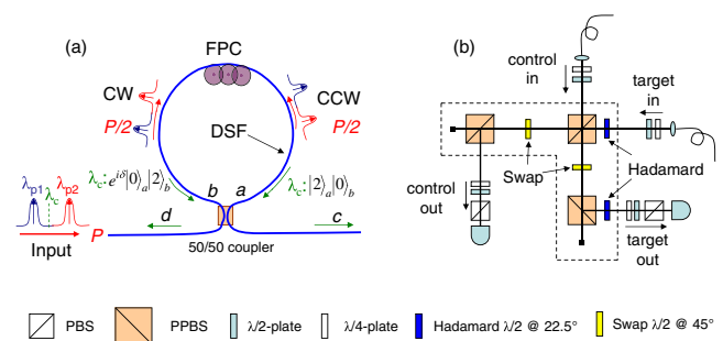
FIG. 1 (color online). Key components of the CNOT gate. (a) QS source. Two identical-photon-pair wave functions interfere at a 50/50 beam splitter with zero phase difference, resulting in deterministic splitting of the photon pair. DSF, dispersion-shifted fiber; FPC, fiber polarization controller; CW, clockwise; CCW, counterclockwise. (b) Structure of the quantum CNOT gate.
