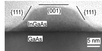
Fig. 1. Transmission electron micrograph of an InGaAs QD grown on a GaAs substrate. Unlike the QDs used in the optical measurements, this dot has not been capped with GaAs.
