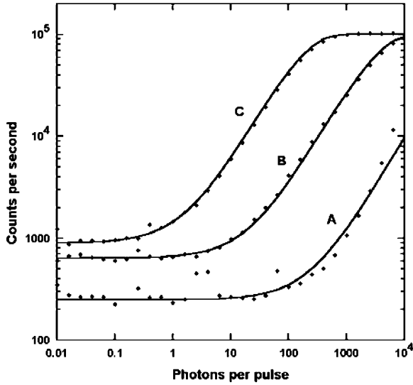
Fig. 12. Determination of SSPD efficiency and dark count rate for three values of bias current. The laser wavelength is 1550 nm and the repetition rate is 100 kHz. For data sets A, B, and C, I_{Bias} is set at 68%, 80%, and 94% of I_C , respectively. The solid curves are fits to the equation given in (2) for dark count rate D and DE \eta . The fits yield values of D = 250 Hz and \eta = 8 \times 10^{-6} for data set A, D = 640 Hz and \eta = 2 \times 10^{-4} for B, and D = 900 Hz and \eta = 5 \times 10^{-3} for C.
