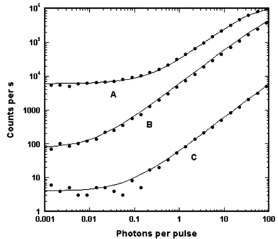
Fig. 14. Determination of efficiency and dark count rate of a second SSPD. The laser wavelength is again 1550 nm, but here the repetition rate is increased to 1 MHz. For data sets A, B, and C, I_{Bias} is set at 96%, 82%, and 65% of I_C , respectively. The solid curves are fits to the equation given in (2) for dark count rate D and DE \eta . The fits yield values of D = 6 kHz and \eta = 2.7 \times 10^{-2} for data set A, D = 75 Hz and \eta = 6 \times 10^{-3} for B, and D = 4.5 Hz and \eta = 6 \times 10^{-5} for C.
