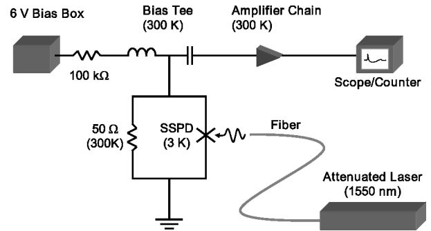
Fig. 10. Schematic of bias and readout circuit.
