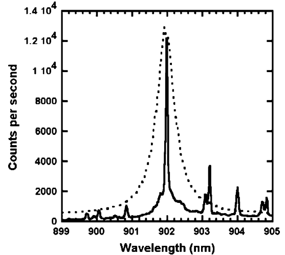
Fig. 17. Emission spectra of cavity-embedded QD at low pump irradiance ( 23 \text{ W/cm}^2 , solid trace) and high pump irradiance ( 206 \text{ W/cm}^2 , dotted trace, magnitude divided by a factor of 50). The QD temperature is 30 K, and the laser is tuned to a central wavelength of 780 nm and emits \sim 1 -ps pulses.
