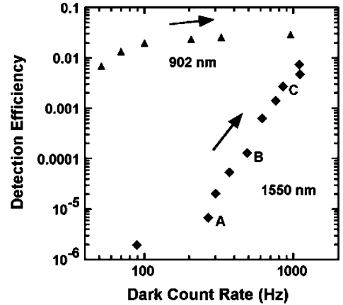
Fig. 13. SSPD system DE versus dark counts at 902 (triangles) and 1550 nm (diamonds). The arrows indicate the direction of increasing bias towards I_C . The data cover the approximate range in I_{Bias} from 60% to 95% I_C . The labels A, B, and C indicate the values determined from the corresponding data sets in Fig. 12.
