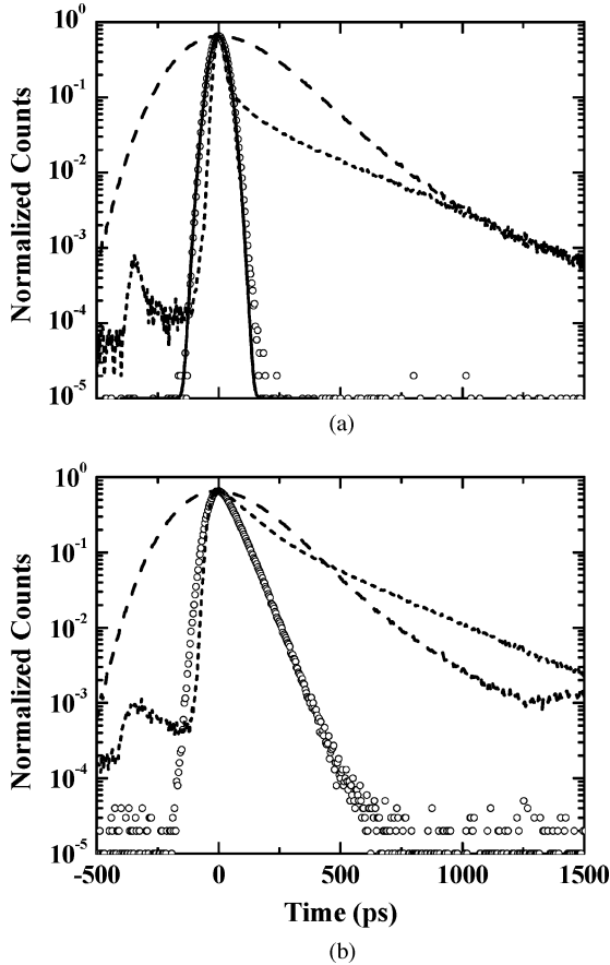
Fig. 15. (a) Instrument response functions of three detectors: SSPD ( open circles ), conventional Si APD ( dashed curve ), and fast Si APD ( dotted curve ). The solid curve is a Gaussian fit to the measured SSPD response function. (b) Lifetime measurement of QW emission at 935 nm with these three detectors. The time axes in (a) and (b) are identical.
