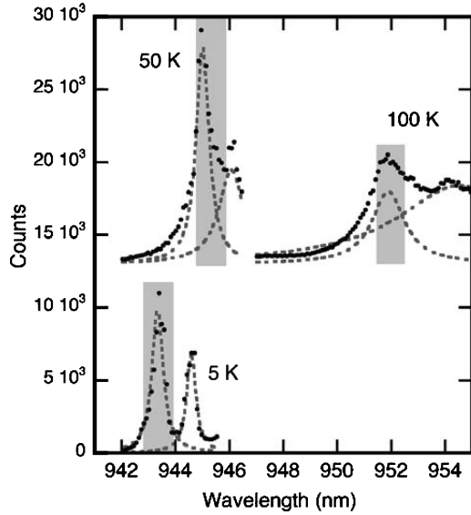
Fig. 6. Measured QD emission spectrum at three temperatures ( solid circles ). Each data set has been fit to a sum of two Lorentzians, and the relative contributions to the fit from the exciton line and the longer wavelength emission line are shown as dashed curves . This longer wavelength line is likely emission from a biexciton or charged exciton state. Each shaded box represents the monochromator position and spectral bandwidth for the corresponding temperature, illustrating the spectral bandwidth of emission incident on the APDs in the HBTI.
