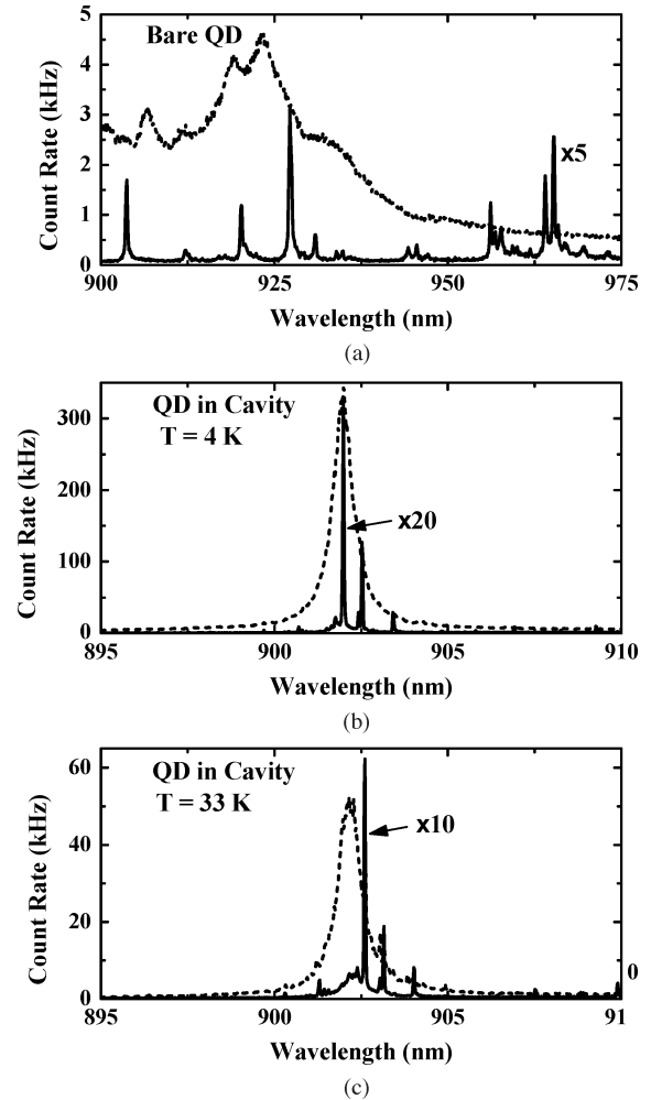
Fig. 7. QD spectra at low and high excitation power, with and without a micropillar cavity. (a) QD in a 2\text{-}\mu\text{m} -wide pillar with no vertical cavity at 4 K for average pump irradiance of 3.2\text{ W/cm}^2 (solid curve) and 10\text{ kW/cm}^2 (dashed curve). (b) QD in a 2\text{-}\mu\text{m} -diameter micropillar cavity at 4 K for 15\text{ W/cm}^2 (solid curve) and 134\text{ W/cm}^2 (dashed curve) average pump irradiance. (c) Same conditions as (b), except for a temperature of 33 K.
