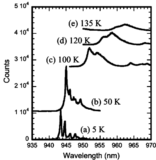
Fig. 4. Temperature-dependent emission spectra from a 2- \mu\text{m} -wide square mesa using a CCD camera with a 10-s integration time. These spectra and the photon correlation measurements shown in Fig. 5 are obtained under identical excitation conditions. The spectra are vertically offset for clarity.
