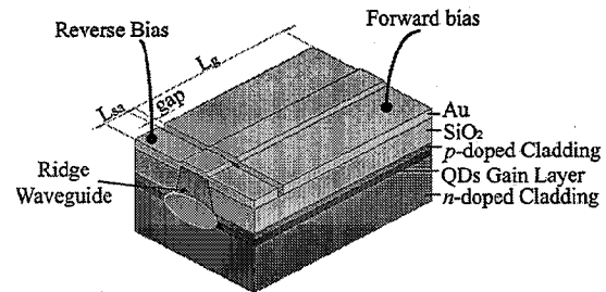
Fig. 1. Schematic of the two-section QD diode laser. Waveguide width = 6 \mu\text{m} ; L_g = 5.5 mm; L_{sa} = 0.3 mm.
