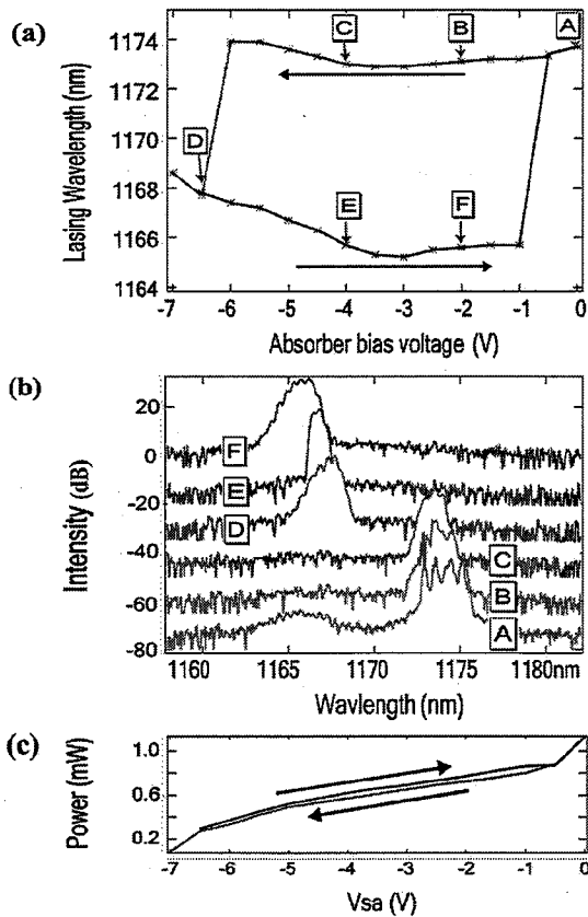
Fig. 2. (a) Wavelength of the laser emission as a function of absorber bias ( V_{sa} ) at a fixed gain section current of 55 mA. The dark (top red) trace is taken with the bias ramped up (down). (b) Optical spectra at various positions in the above hysteresis curve (the curves are offset for clarity). (c) Optical power as a function of V_{sa} .
