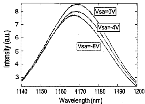
Fig. 4. Electroluminescence spectra taken from a sample similar to the laser, but with an antireflection coating to inhibit lasing. The light was extracted from the facet adjacent to the absorber region. V_{sa} is the bias voltage of the absorber region.
