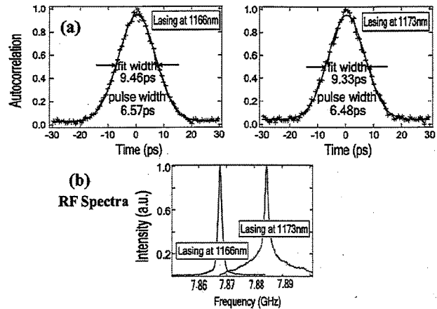
Fig. 3. (a) Intensity autocorrelation for the mode-locked pulses on different branches of the hysteresis curve, both at -4 -V reverse bias. (b) Corresponding radio-frequency spectra.
