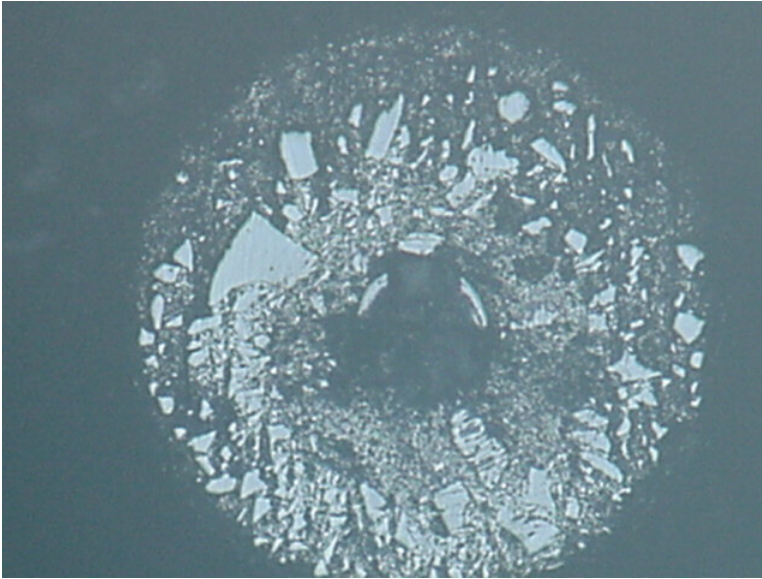
Figure 9. Magnified optical image of biconic optical fiber connector endface showing the surface contamination.
