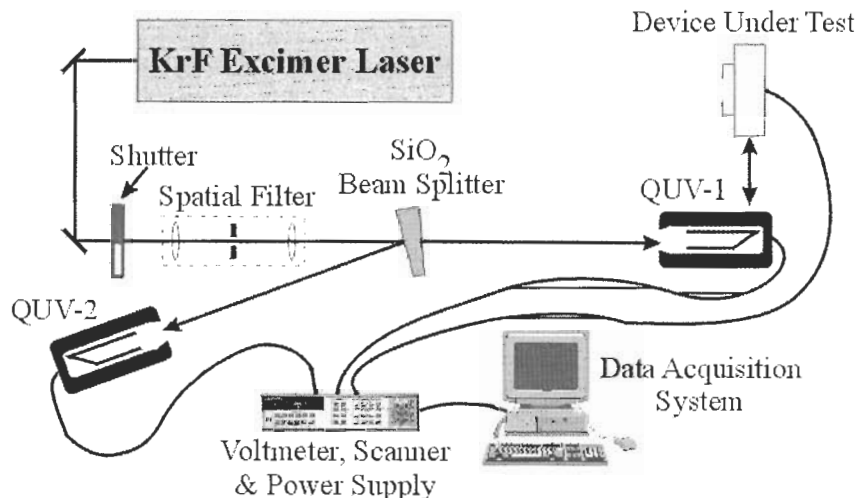
Figure 3. KrF excimer laser measurement system.
