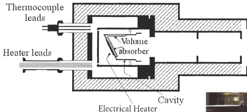
Figure 2. Schematic drawing of NIST 193 nm calorimeter.
