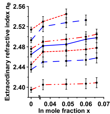
Fig. 4 (b) Extraordinary refractive index of \text{In}_x\text{Ga}_{1-x}\text{N} over the same wavelength and x values as used in (a).
