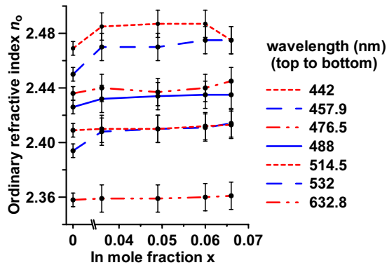
Fig. 4 (a) Ordinary refractive index of \text{In}_x\text{Ga}_{1-x}\text{N} for the wavelengths indicated. The values for x were given earlier. Refractive index values for GaN ( x = 0 ) are taken from Ref. [1].
