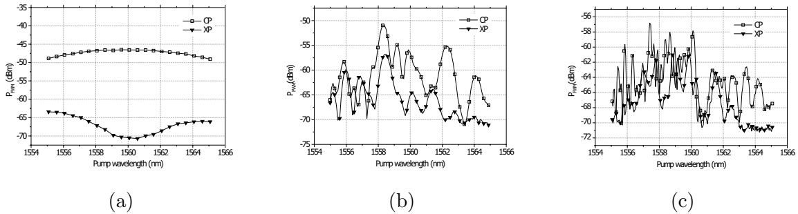
Figure 3: Measured FWM efficiency with parallel and crossed input SOPs: (a) \Delta\lambda = 1 nm, (b) \Delta\lambda = 5 nm and (c) \Delta\lambda = 8 nm
