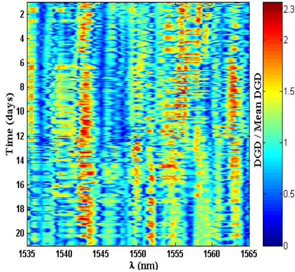
Figure 2. Measured, normalized DGD vs. wavelength and time for 2-3 fiber concatenation (21 days of data).
