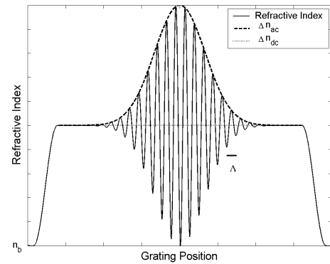
Figure 2. Physical interpretation of \Delta n_{ac} , \Delta n_{dc} , and \Lambda of a FBG. An un-chirped Gaussian apodized FBG shown. The modulation frequency is not shown to scale. n_b : fiber bulk index.
