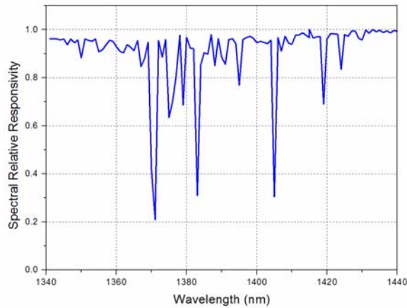
Figure 5: Spectral relative responsivity of the radiometer in the water vapour absorption region.
