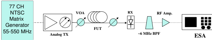
Fig. 7. Analog transmission experimental setup
