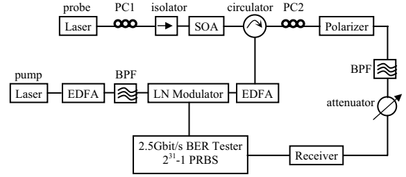
Fig.5. Experimental setup for all-optical wavelength conversion based on XPolM.
