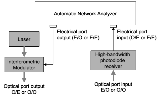
Figure 1 General configuration of an optical ANA
