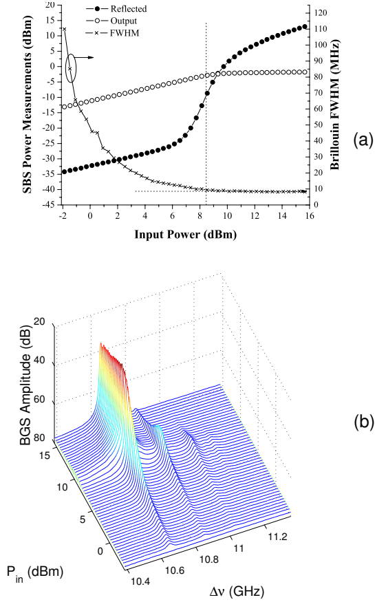
Fig. 3. (a) SBS threshold measurements for an NZ-DSF overlaid with FWHM data from above data. The vertical line represents the boundary from spontaneous to stimulated Brillouin scattering and the onset of SBS-induced pump depletion. (b) Measure Brillouin gain spectrum at various input powers using the configuration in Fig. 2.
