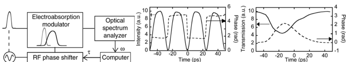
Fig. 3: spectrogram implemented using an electroabsorption modulator as a gate (left). The computer controls the delay between the gate and the pulse using a RF phase shifter operating on the driving signal to the EAM and records the spectra after modulation. Measured electric field of a CSRZ train of pulses (middle) and measured transmission of a gain-depleted SOA (right).
