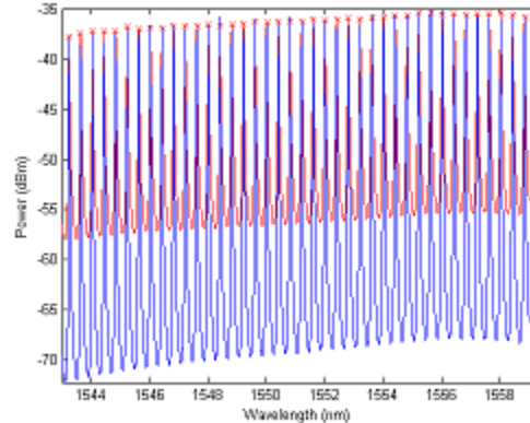
Figure 5 A comparison between a Unprocessed raw spectrum (Red), which consists of more than 40 50-GHz-spacing DWDM channels, and the deconvoluted spectrum (blue).
