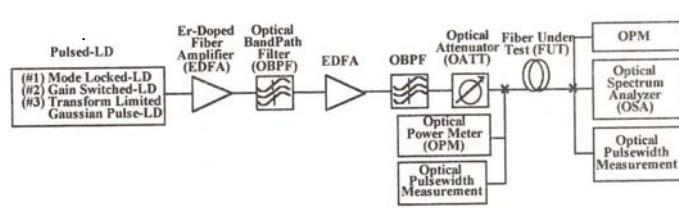
(a) Pulsed-LD SPM (P-SPM)
