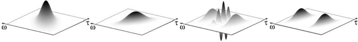
Fig.1: Wigner-Ville function of a Fourier-transform limited pulse, a chirped pulse, 2 mutually coherent chirped pulses and 2 mutually incoherent chirped pulses (from left to right). In the latter case, note the absence of the crossed terms between the two individual Wigner functions.
