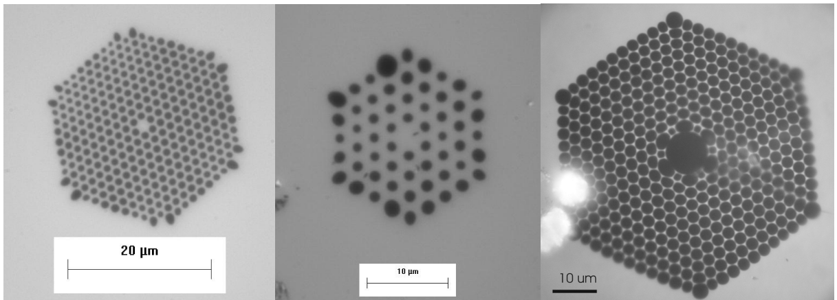
Fig.1: The analyzed microstructured fibers: 2µm core PCF, 3.5µm core PCF, and air-guiding bandgap fiber
