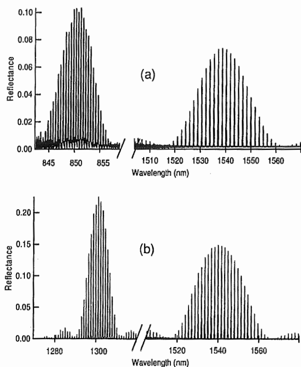
Fig. 1. Reflection spectra of ISFBGs, measured with an optical spectrum analyzer with superluminescent diodes used as light sources. (a) Spectrum of an ISFBG with 850- and 1550-nm peaks. (b) Spectrum of an ISFBG with 1300- and 1550-nm peaks.
