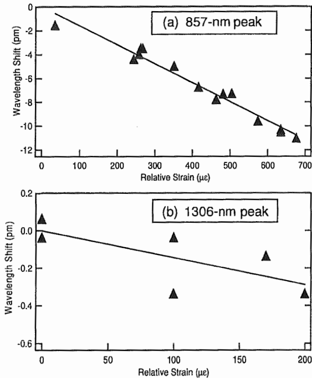
Fig. 3. Wavelength of stabilized grating as strain is applied ( 1 \mu\epsilon = 1 \times 10^{-6} ). (a) The 857-nm peak of the 850- and 1550-nm ISFBG. (b) The 1306-nm peak of the 1300- and 1550-nm ISFBG.
