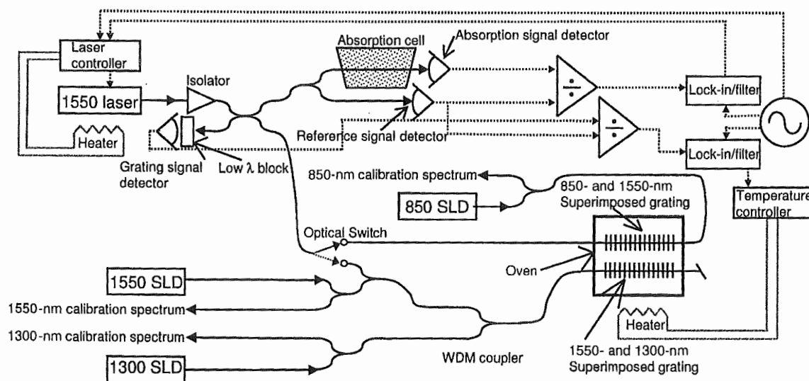
Fig. 2. Diagram of the hybrid wavelength reference. The upper section contains the components used to stabilize both a laser to a HCN line and a 1550-nm grating peak to this laser. The lower section contains the ISFBGs. Superluminescent diodes (SLDs) illuminate the fiber gratings, and the light reflected off the gratings is observed at the calibration spectrum ports. An optical filter prevents 850-nm SLD light from reaching the grating signal detector. WDM, wavelength division multiplexing.
