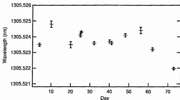
Fig. 4. Wavelength of a 1300-nm wavelength reference peak over 70 days.
